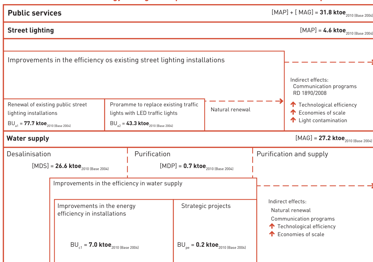
Chart 47. Breakdown of energy saving in the public service sector in 2010 with respect to 2004
