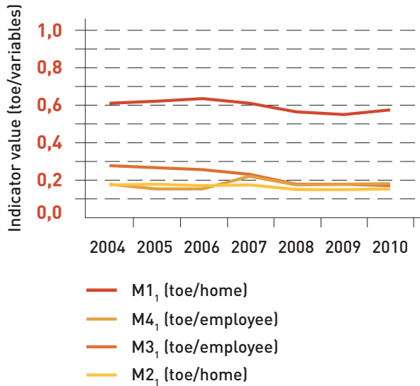
Chart 31. Evolution of “M” indicators related to envelope and thermal installations use in the period 2004-2010
