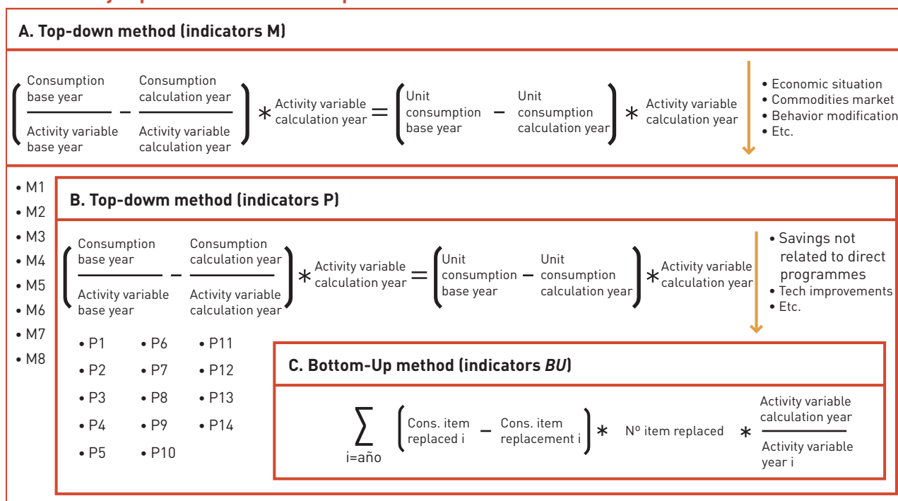
Chart 2. Diagram of the methodology for energy savings calculation, which combines consistently top-down and bottom-up indicators
