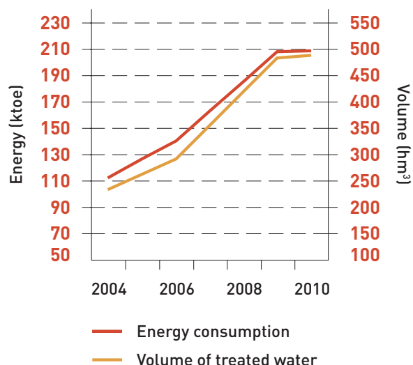
Chart 52. Evolution of electric power consumption related to desalination and volume of treated water in the period 2004-2010
