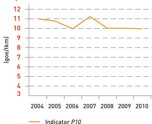
Chart 16. Evolution of "P10" indicator related to passenger railway transport in the period 2004-2010
