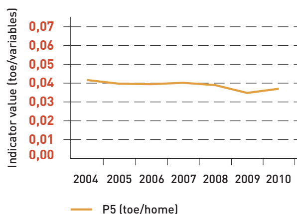
Chart 41. Evolution of "P" indicators related to interior lighting use in the period 2004-2010
