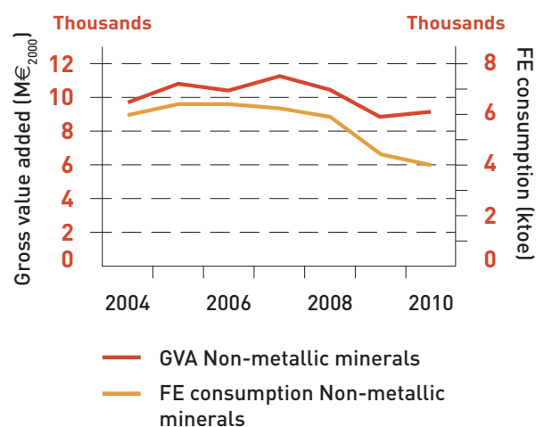
Chart 6. Evolution of final energy consumption and Gross Value Added in the "Non-metallic minerals" activity in the period 2004-2010
