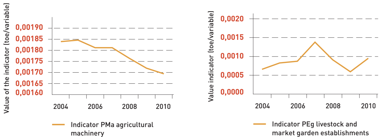
Chart 63. Evolution of “P Ma ” and “P Cl ” indicators in the period 2004-2010
