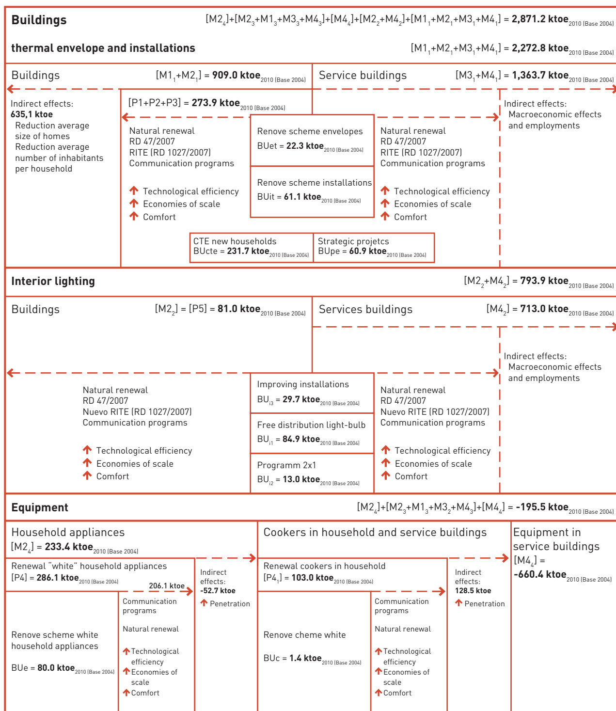
Chart 26. Breakdown of energy saving in the building sector in 2010 with respect to 2004
