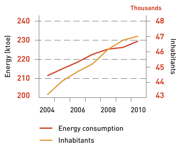
Chart 53. Evolution of electric power consumption related to treatment and number of inhabitants in the period 2004-2010
